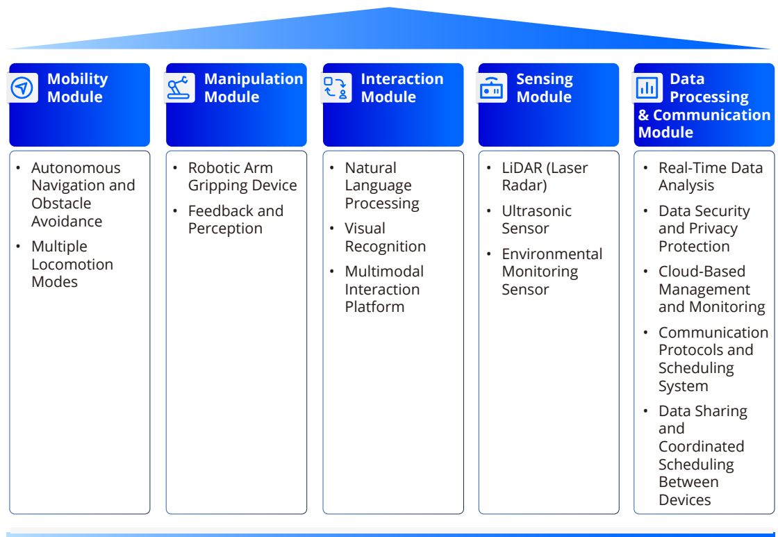
Figure 2-2: R2X modular design architecture
